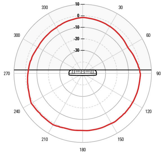
ELEVATION 2.4 GHZ
