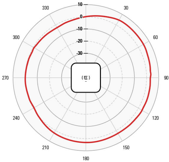
AZIMUTH 2.4 GHZ
